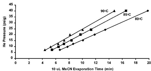
Figure 1. Evaporation time of 10 \mu\text{L} of MeCN in DSI with the ChromatoProbe with respect to injector temperature and He pressure.
